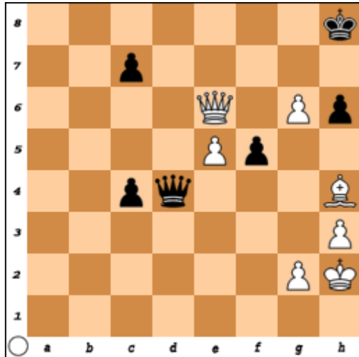
Diagram 6. Leon - Ebe, slotstelling na 41. g6
