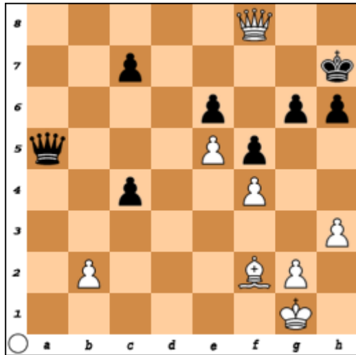
Diagram 4. Leon - Ebe na 34. Dxf8
